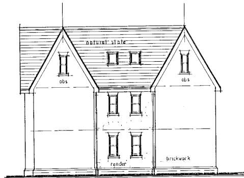
NORTH-EAST ELEVATION
