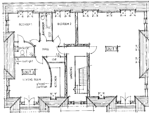
SECOND FLOOR LAYOUT
